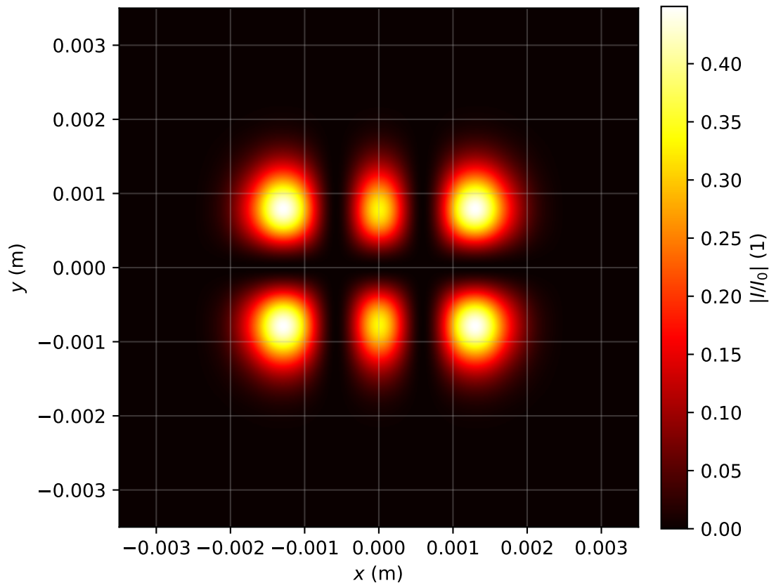
Intensity profile I(x, y, z = 2.548)/I_0 , P_{in}=1.0P_{cr} , artificial time
